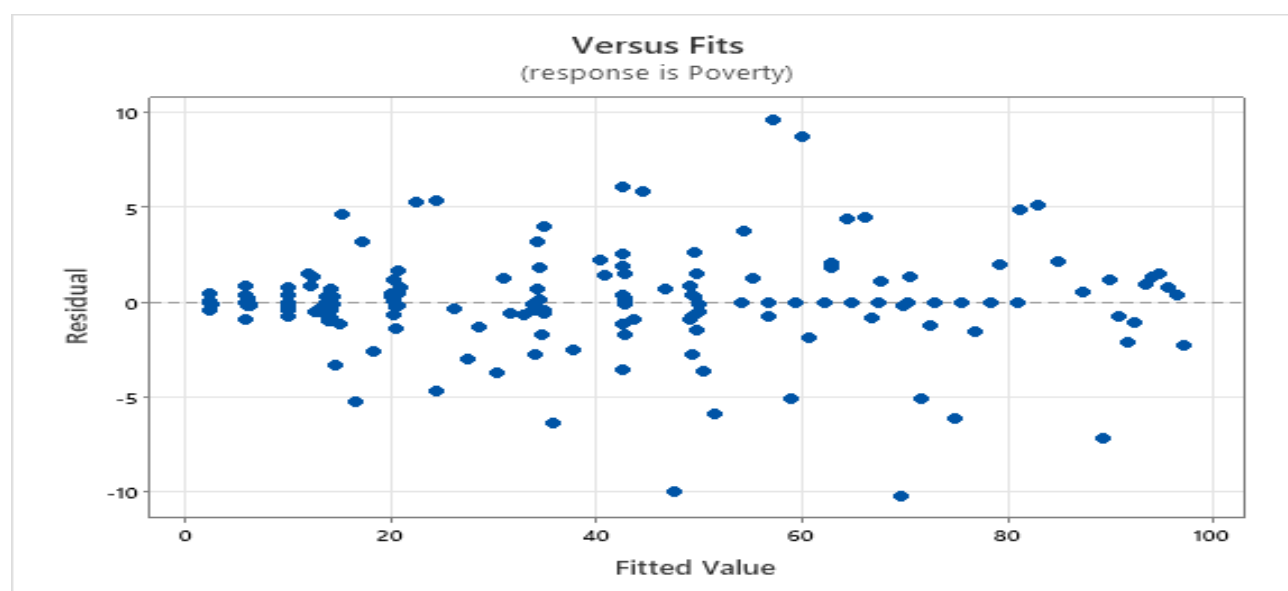
Figure 3: Plot of the Predicted value Against the Residual
