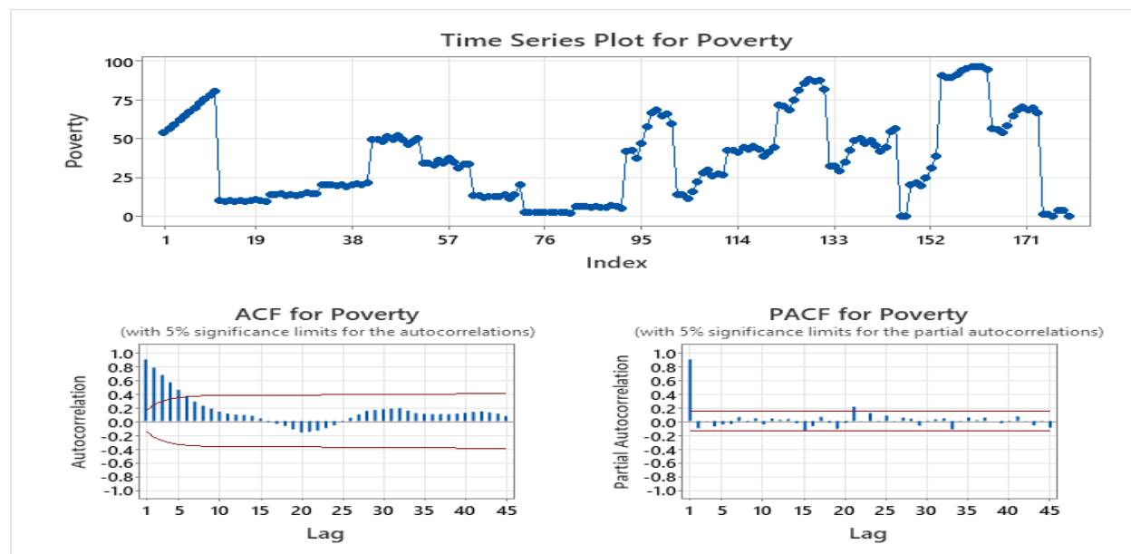
Figure 1: ACF and PACF Plots for Poverty Rates
