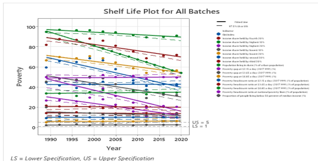
Figure 2: Shelf-Life Plot for all Indicators (Batches)
