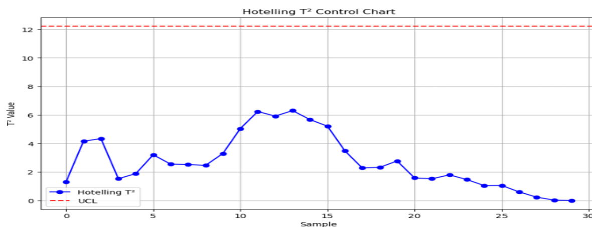
Figure 1: Hotelling T^2 Control Chart
