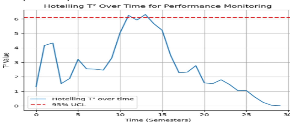
Figure 2: Plot of Hotelling T^2 Over Time for Performance Monitoring
